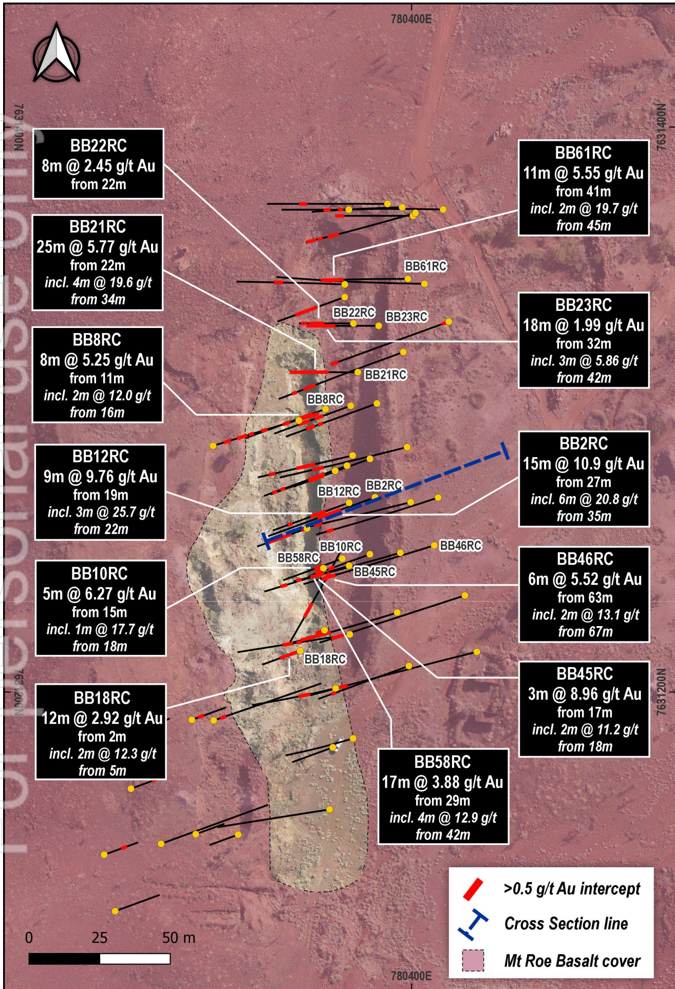
Figure 2- Plan view of Blue Bar
