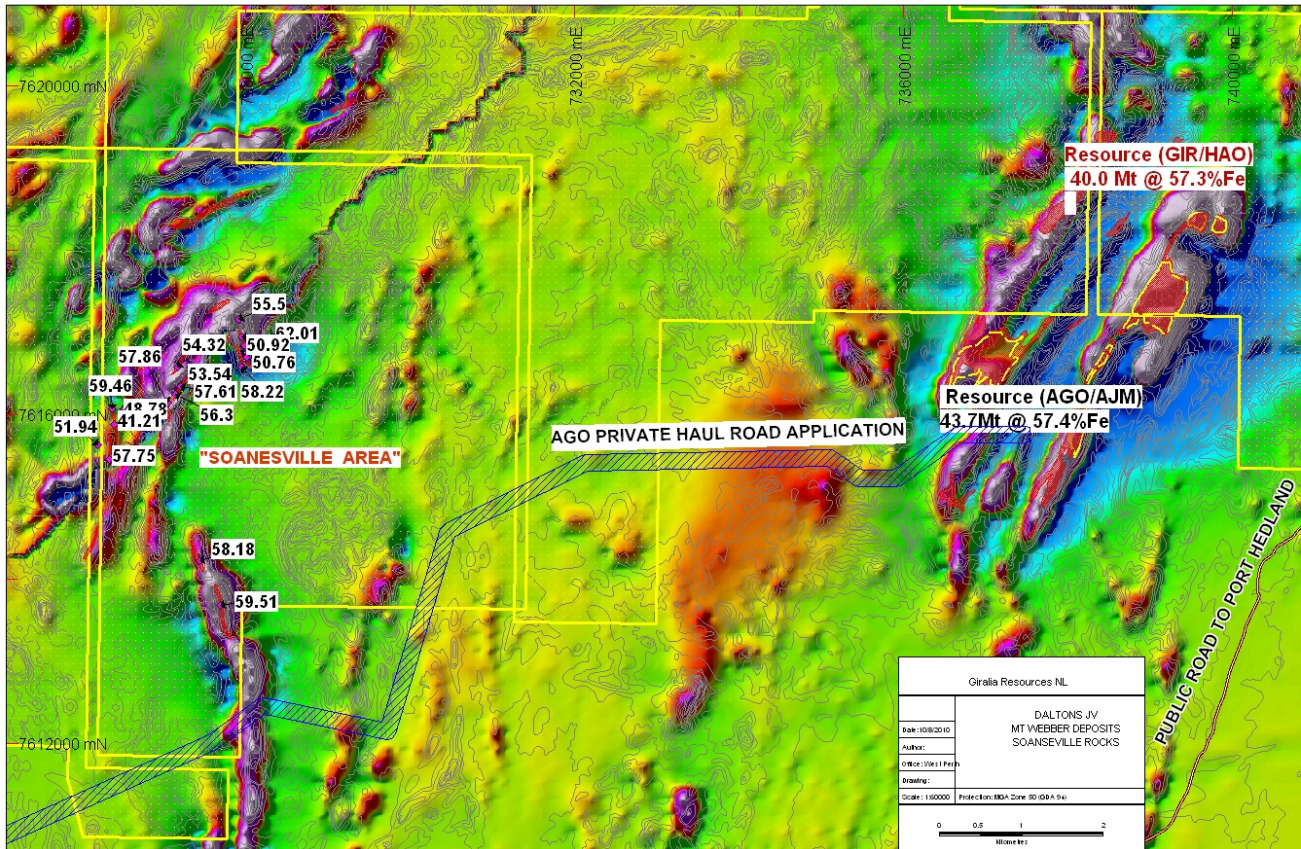
Figure 3: Daltons JV eastern portion aeromagnetic image, showing Mt Webber deposits and new Soanesville area sampling results (Fe %).
